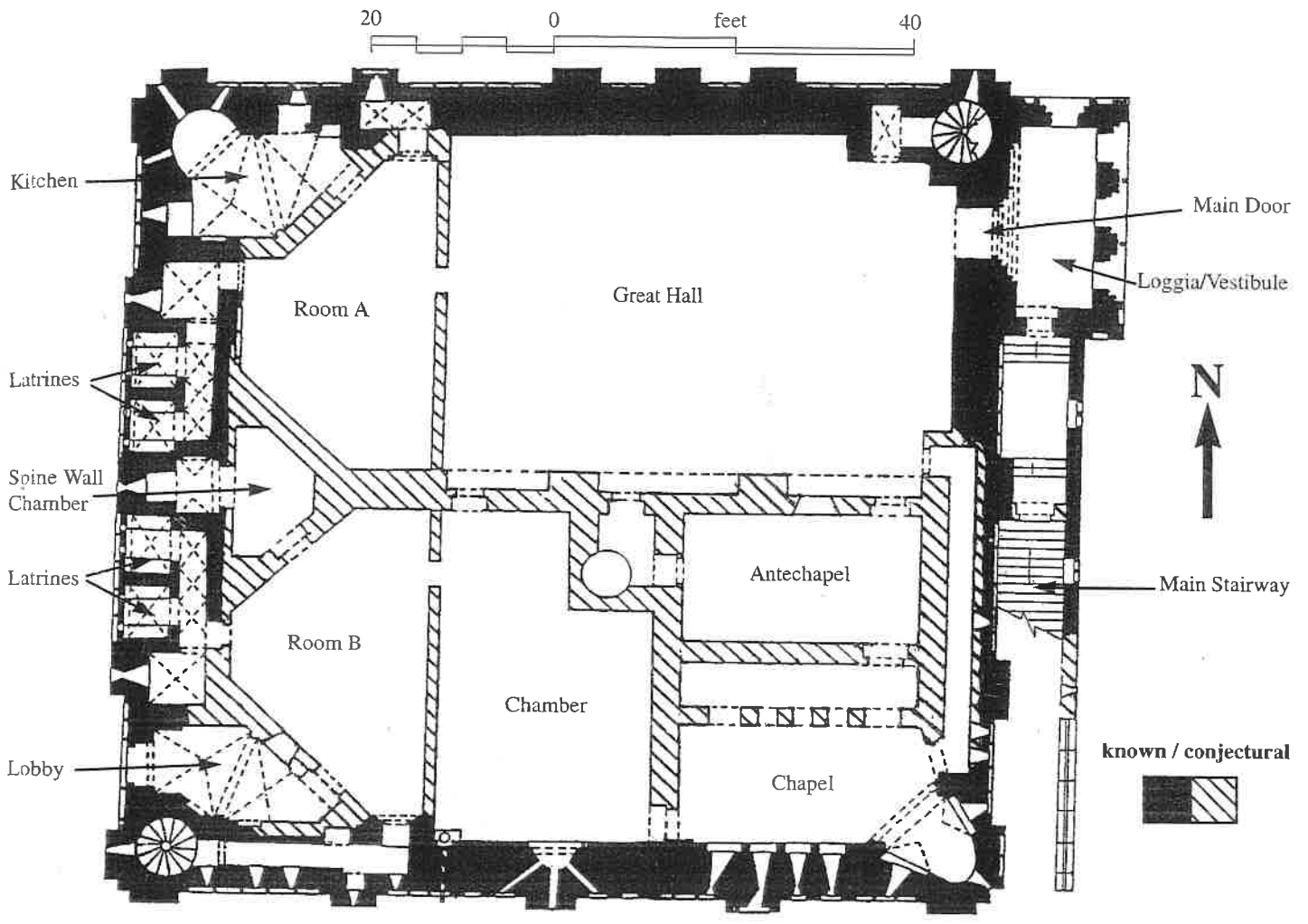
16) Plan of the main floor of Norwich keep
